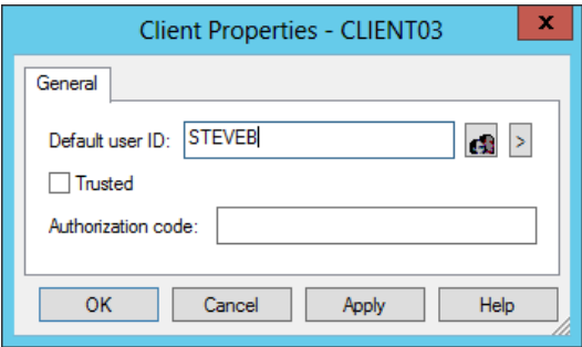
Figure 31 Client Properties
