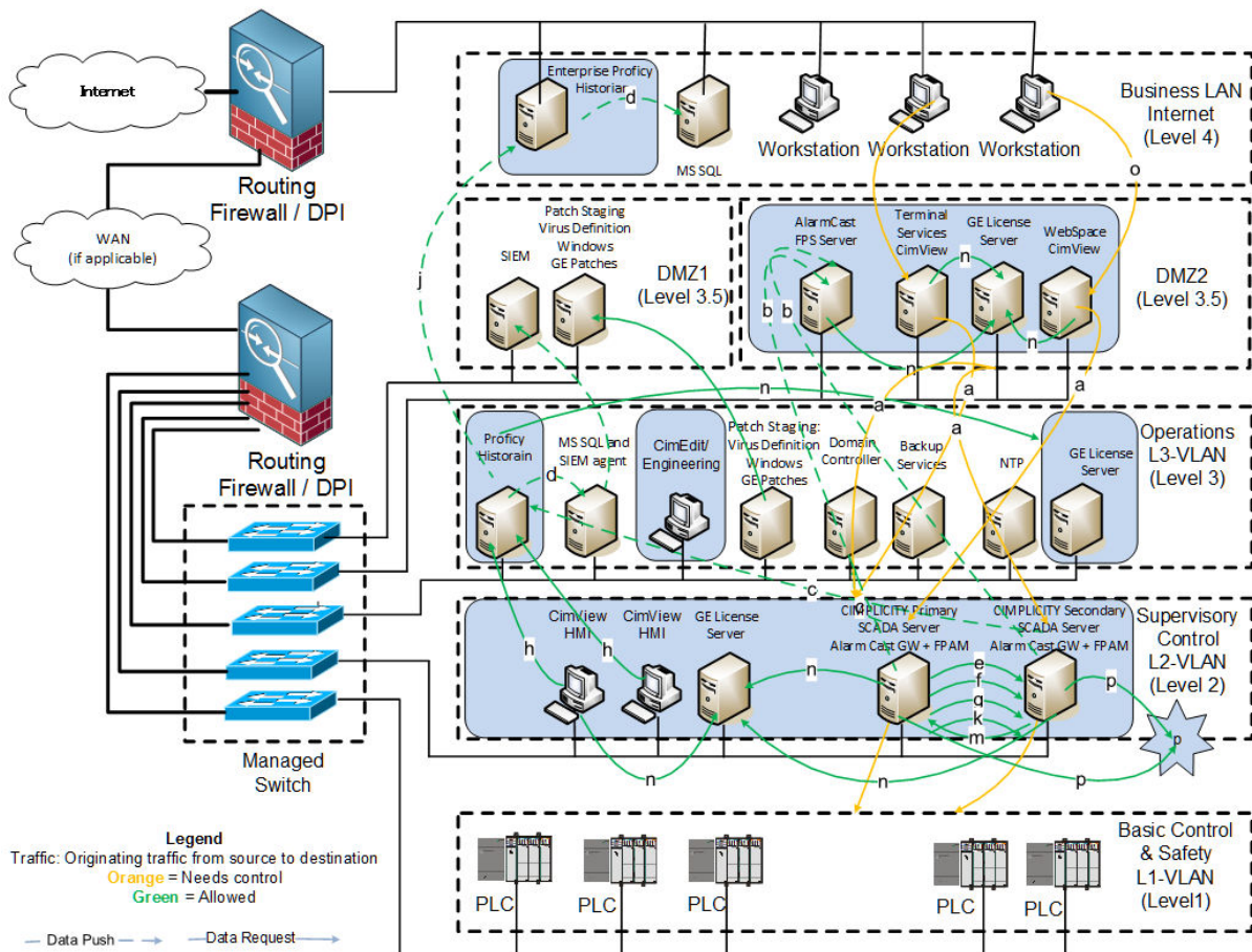
Figure 4 Remote Access to CIMPLICITY Screens with WebSpace Solution and Terminal Services Solution
